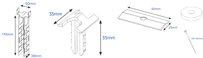
10 Galvanised batten brackets; 26 ridge union clips; 13 clamping plates; 13 EPDM washers; 13 screws
